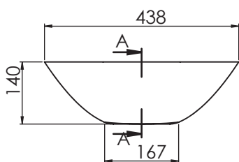
VISTA FRONTAL
