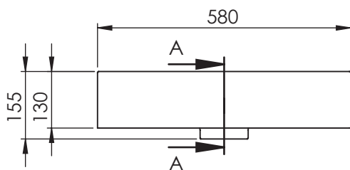
VISTA FRONTAL
