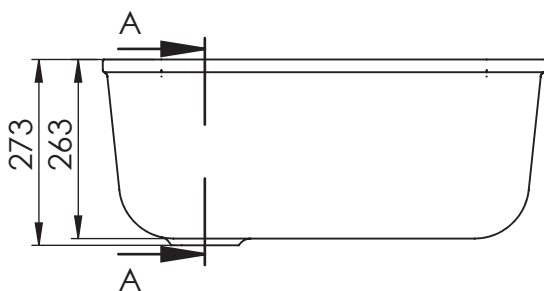
VISTA FRONTAL
