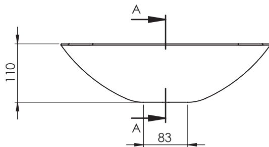
VISTA FRONTAL
